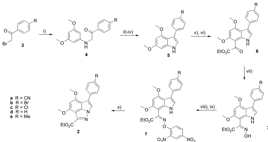
Scheme 3. Syntheses of the tricycles 2a–e . Reagents: (i) 3,5-dimethoxyaniline, EtOH, NaHCO 3 , Δ; (ii) (CF 3 CO) 2 O; (iii) CF 3 CO 2 H; (iv) KOH, MeOH; (v) (COCl) 2 ; (vi) EtOH; (vii) NH 2 OH·HCl, pyridine, EtOH, Δ; (viii) Na, EtOH; (ix) 2,4-fluorodinitrobenzene; (x) NEt 3 , THF, Δ.
