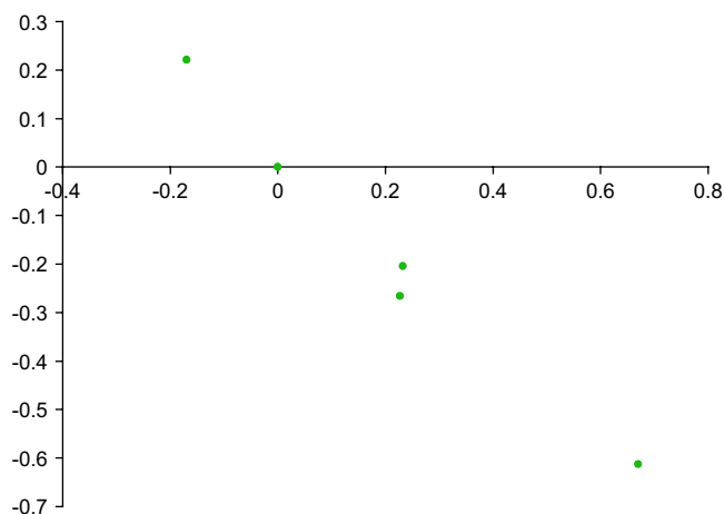
Figure 1. Hammett plot for the cyclisation of the precursors 1a–e under the conditions outlined in Scheme 1.
