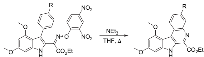
Scheme 2. Cyclisation of ethyl 3'-aryl-4',6'-dimethoxyindol-2'-yl-2-(hydroxyimino)acetates, which has been shown to proceed through an electrocyclic mechanism. 2
