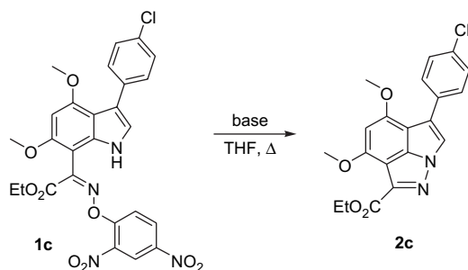
Scheme 1. Cyclisation of the oxime ether 1c to give the corresponding tricycle 2c .
