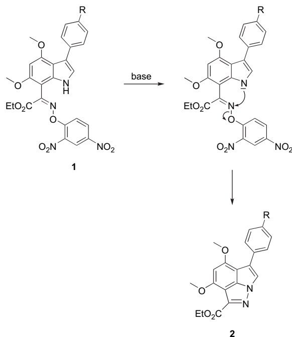
Scheme 4. Cyclisation of the precursors 1 proceeding through a concerted intramolecular substitution.
